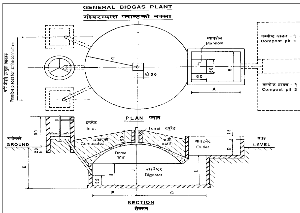
Figure 2: Biogas Model GGC 2047
